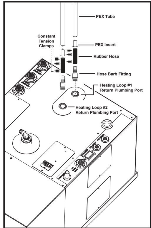
“Return” Heating Loop Ports
