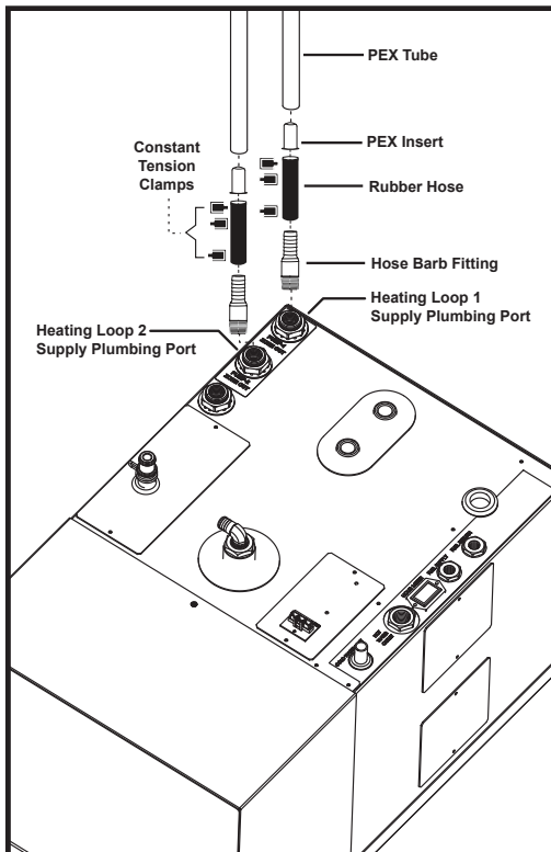
“Supply” Heating Loop Ports
